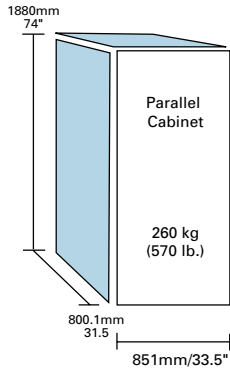
Powerware Hot Sync - Redundant
