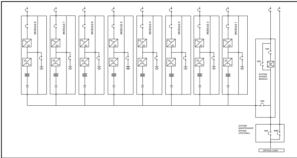
Typical Powerware 9315 200 to 750 kVA Hot Sync Capacity Application
