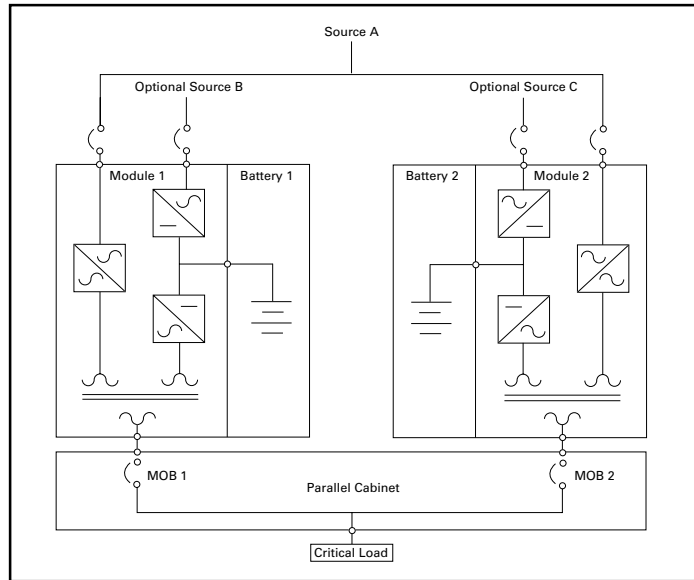
Typical Powerware 10 to 500 kVA Hot Sync Redundant Application
