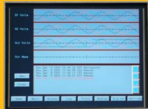
Waveform capture and event capture screen
